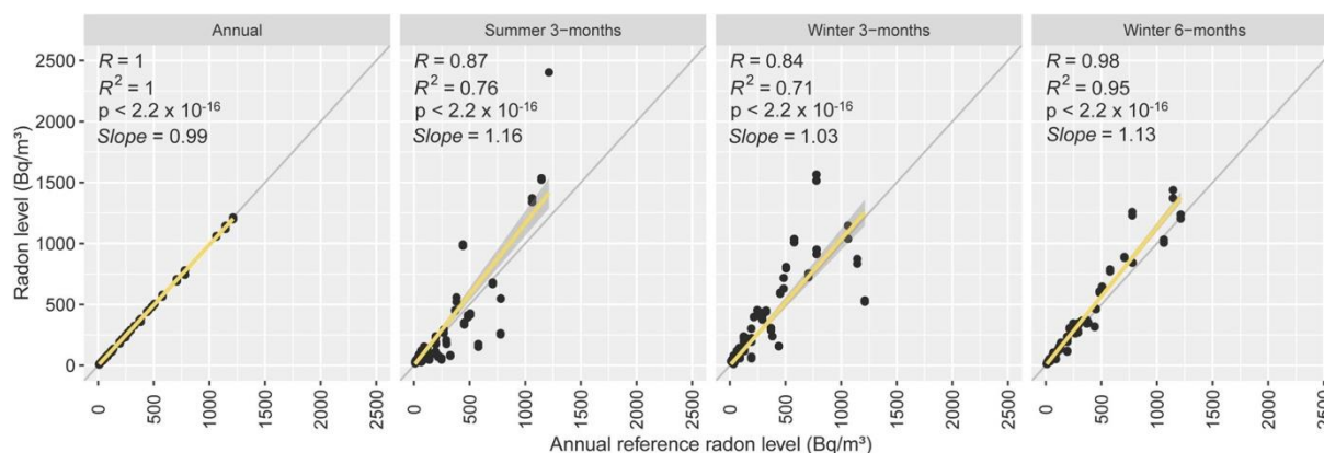
Figure 12: Direct comparison of passive radon measurements of different durations with the annual measurement (taken from Rey et al., 2025)
