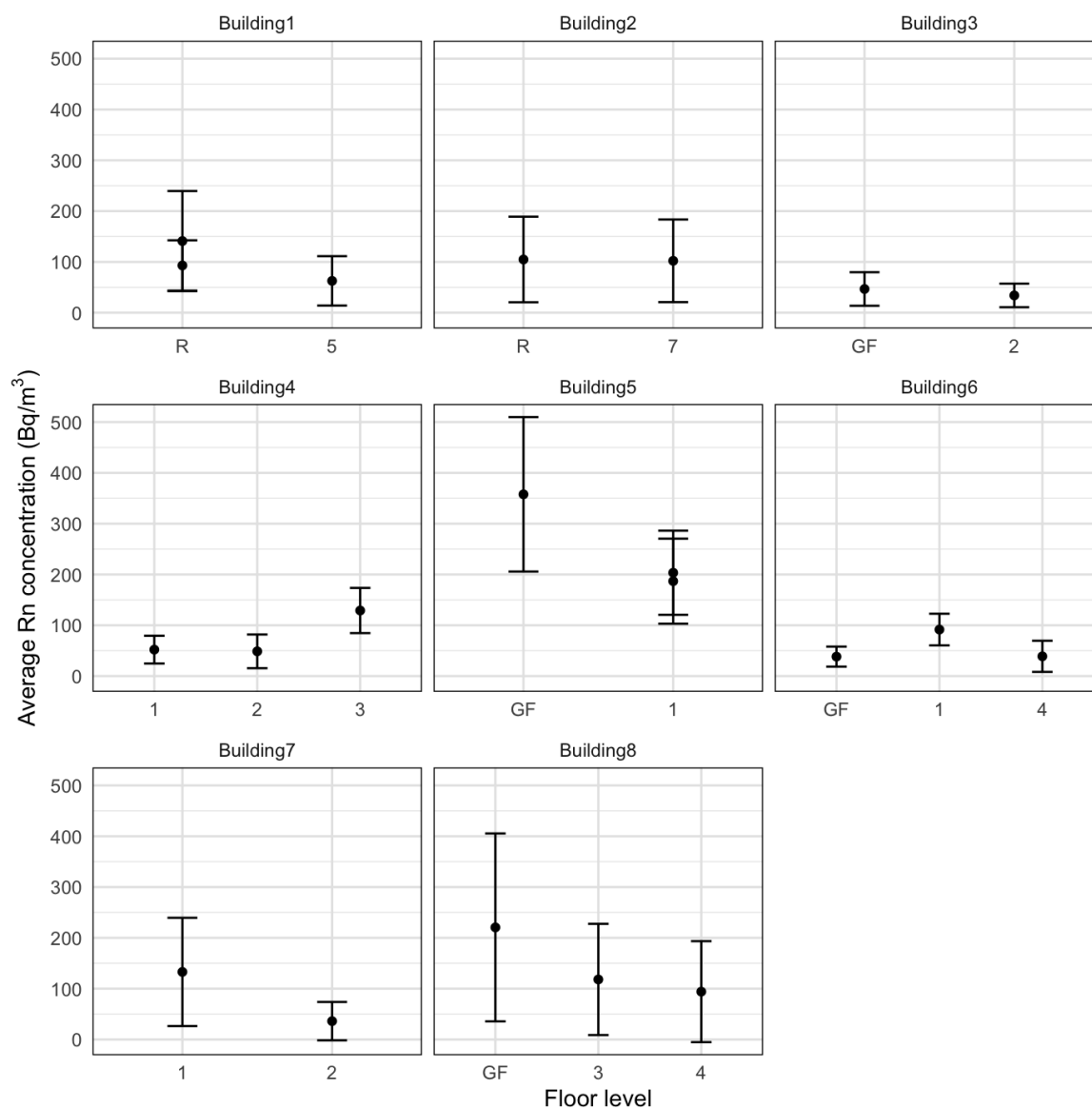
Figure 33: Average annual radon concentration for each measured apartment (± standard deviation) in each building
