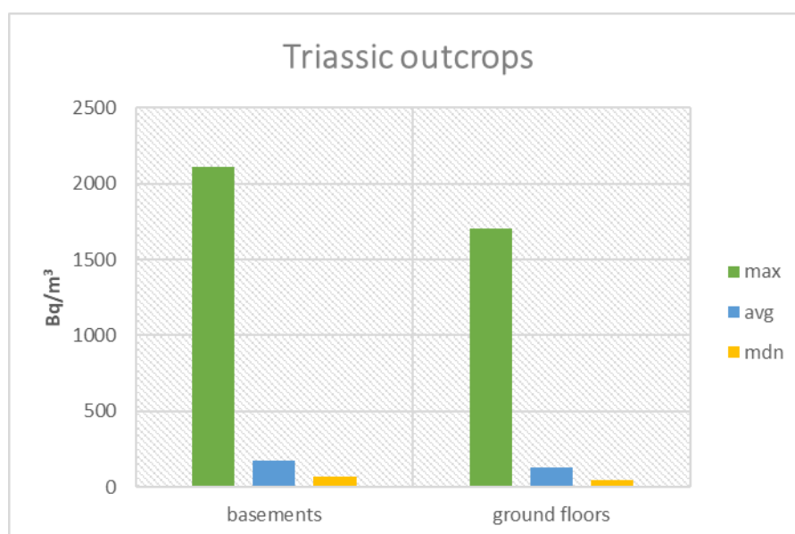
Figure 40: Radon concentrations in buildings located on Triassic outcrops.
